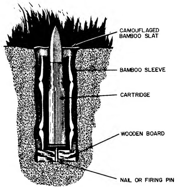
Figure 59. Cartridge trap.
